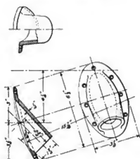
Figs. 3242-3244. Sand Pipe Cover on Sandbox Casing.
